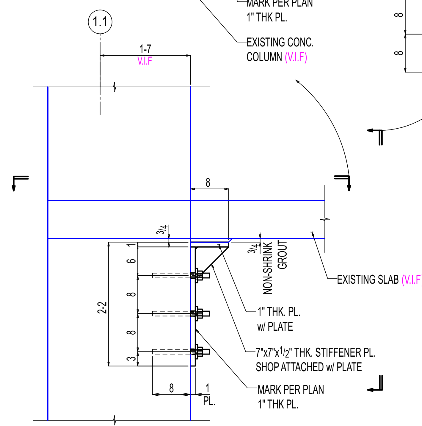
A-A E-12.00 (REF:4/S317) OTHERS NOT SHOWN FOR CLARITY
