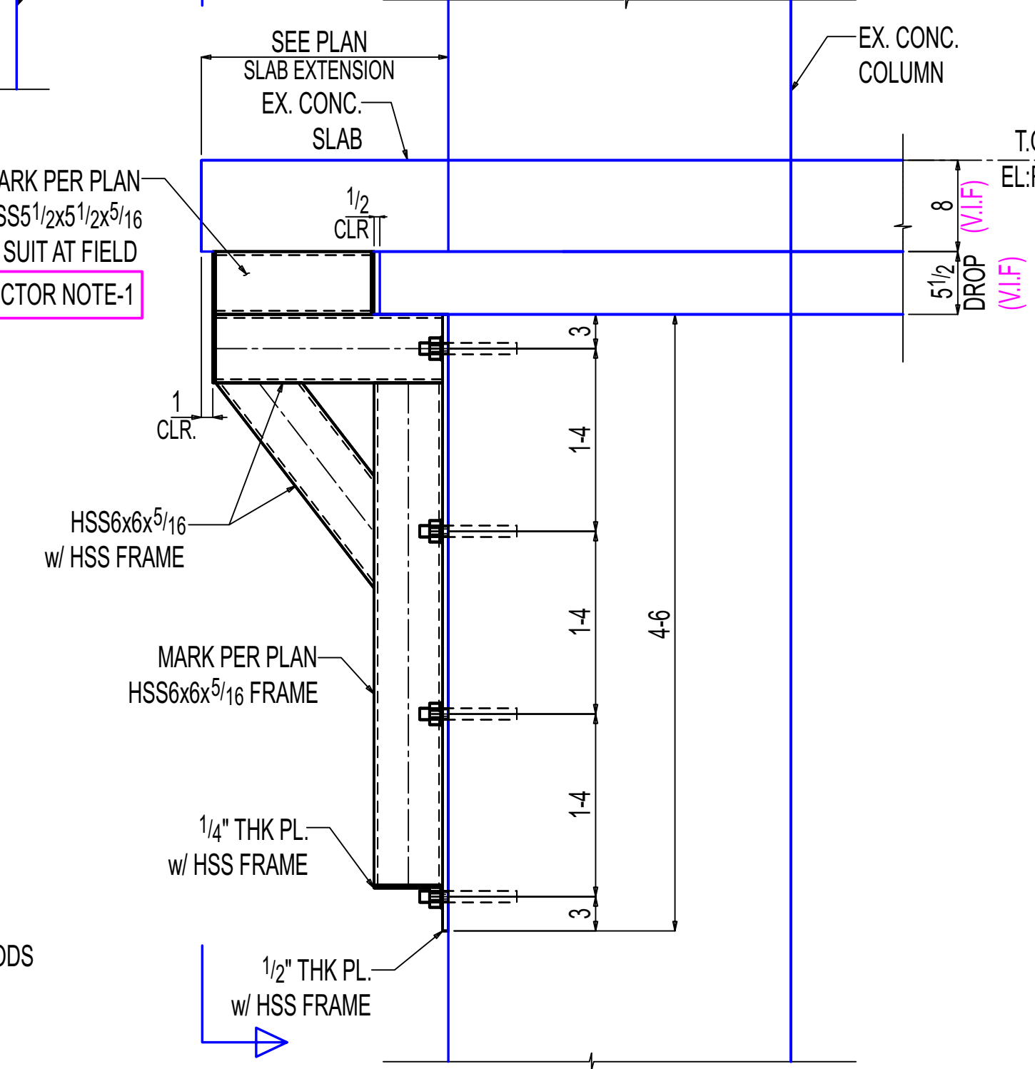
B-B (NEW SLAB EXTENSION SUPPORT (1'-6" TO 3'-10")) E-12.00 (REF:3/S307) OTHERS NOT SHOWN FOR CLARITY
