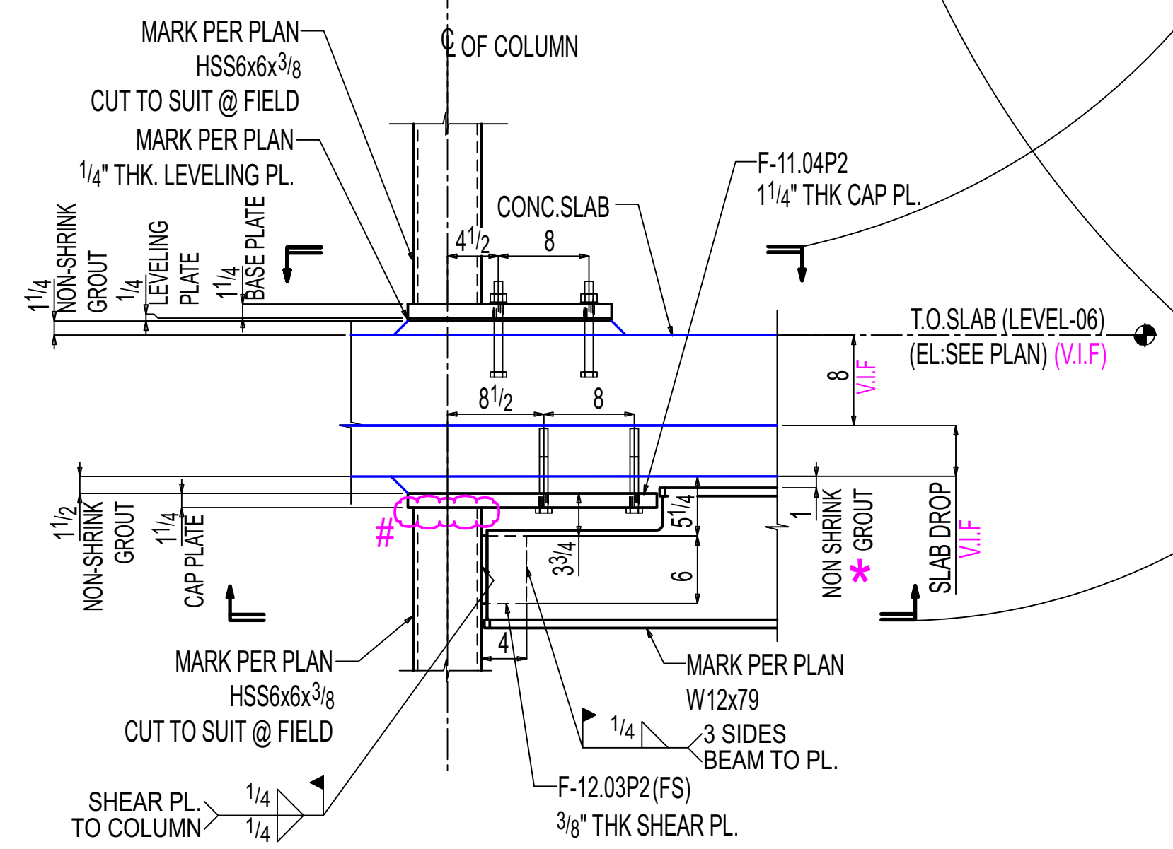
C-C E-12.00 (REF:5.6 & 7/S314) OTHERS NOT SHOWN FOR CLARITY
